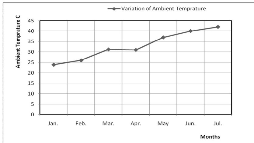
Figure (2) shows region variation of ambient temperature from January to July in Mourzuq area.
